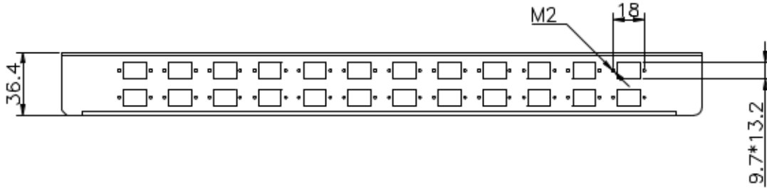
24 Port for SC Simplex Adaptor
