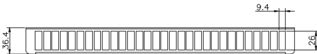
30 Port for LC Quad Adaptor
