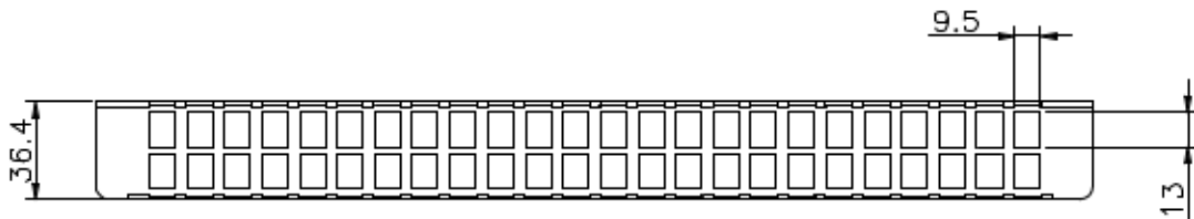
48 Port for SC Simplex Adaptor
