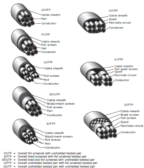
Shielded and unshielded balanced twisted-pair cable design examples
